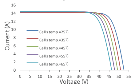
Current-Voltage (590W)
